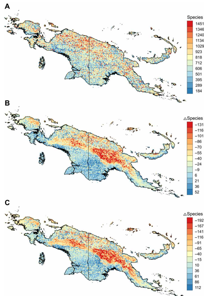
Fig. 1. Endemic plant species richness (number of species per grid cell) in the face of climate change. Species richness under current climate (A) and difference in species richness between current climate and 2070 RCP 2.6 (B) and 2070 RCP 8.5 (C).
